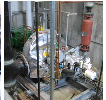
SMALL BACKPRESSURE T-G PACKAGE
